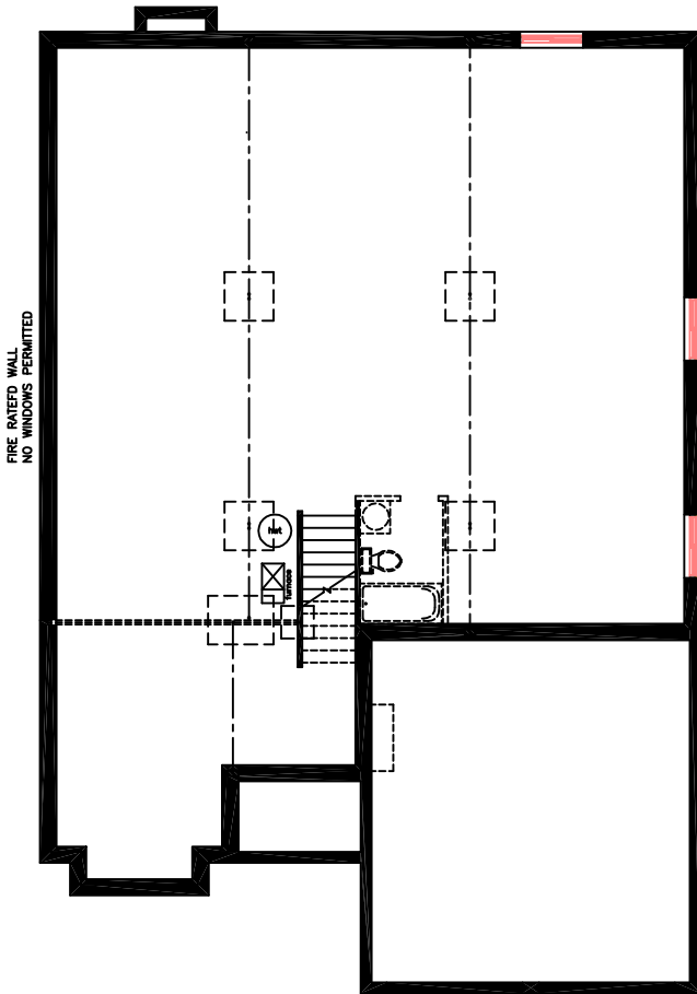
Basement level
