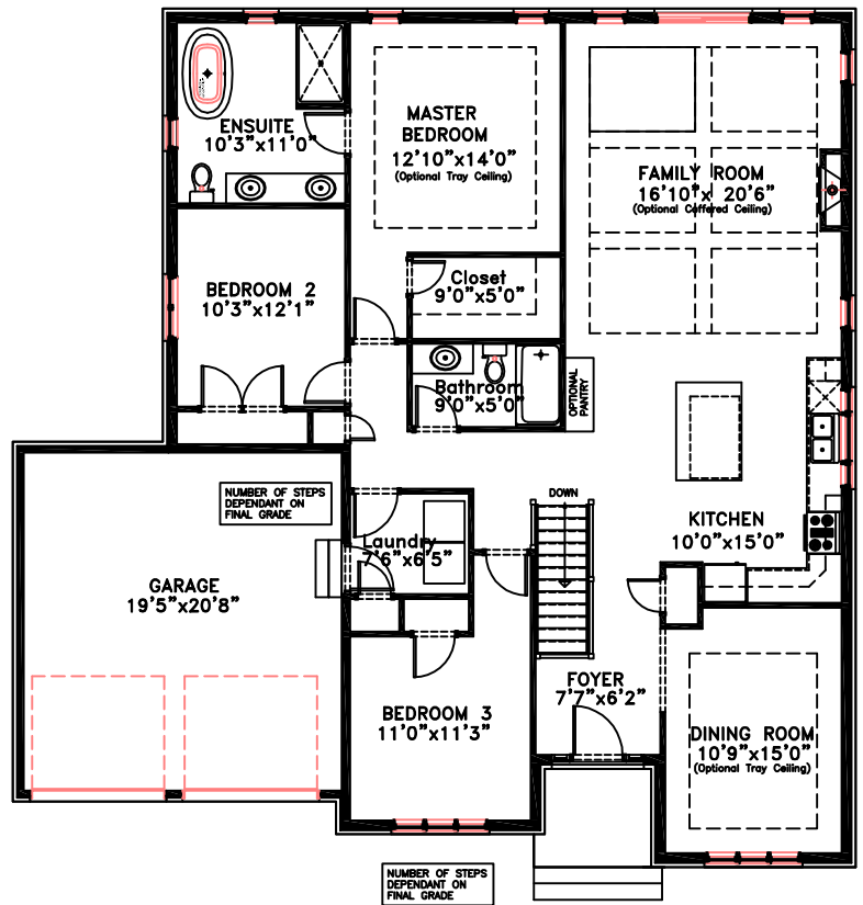
Main Floor level
